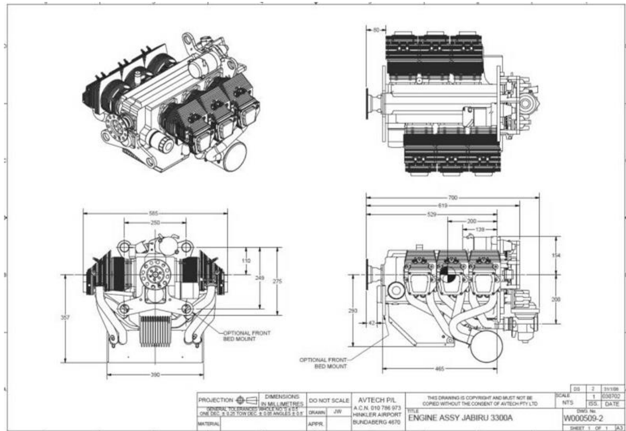
Figure 4 – 3300 Engine Dimensions
