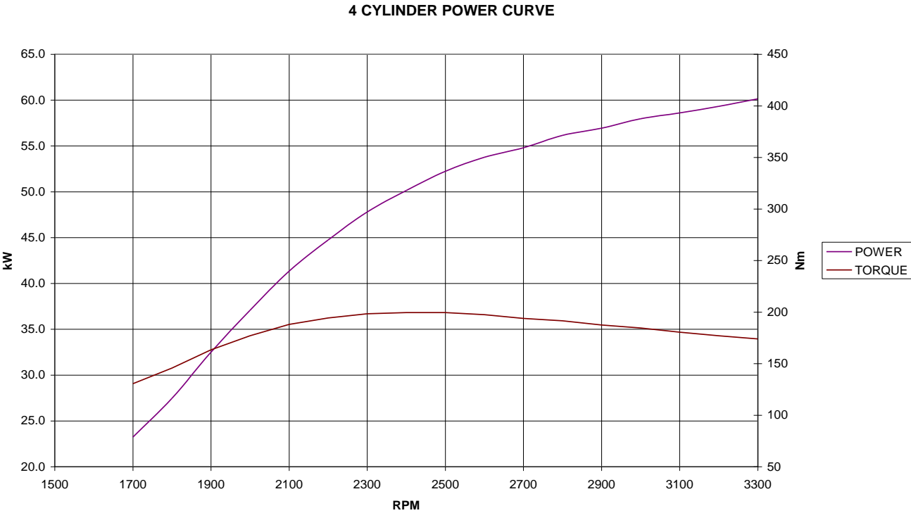
Figure 8 – Power Curve - Typical 2200C, 2200B, Engine
