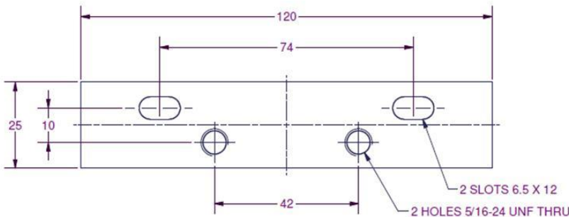
Figure 17 – Dimensional Details For Lifter Tool
