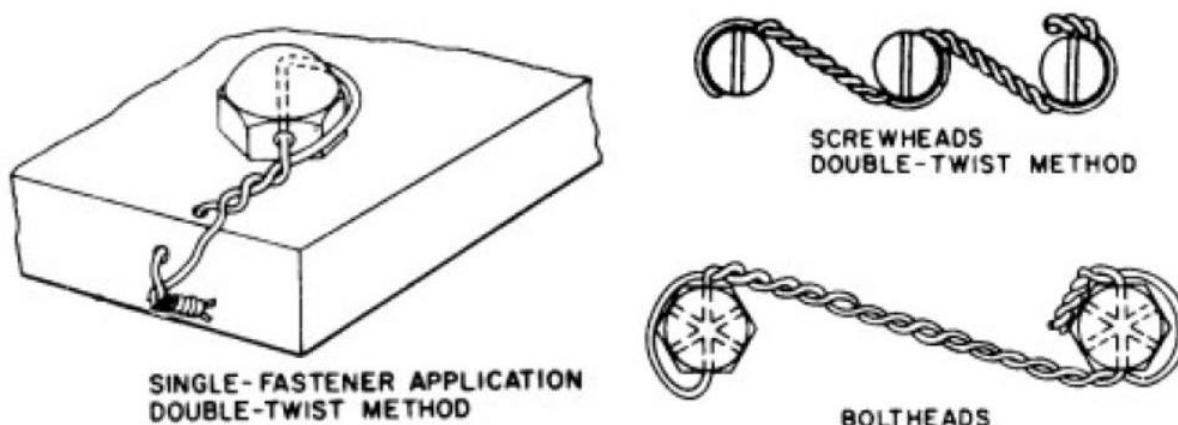
Figure 47 – Safety Wire Details
