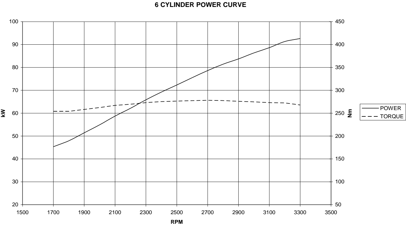
Figure 9 – Power / Torque Curves – Typical 3300 Engine
