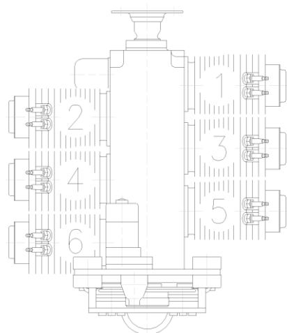
Figure 5 – 3300 Cylinder Denomination
