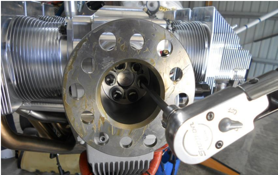
Figure 207 - Installing the Propeller flange
