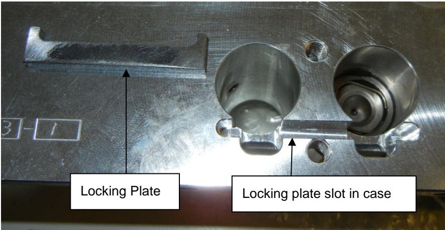
Figure 58 – Crankcase & Locking Plate
