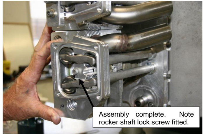
Figure 195 – Fitting Rockers #3
