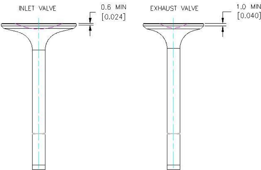
Figure 90 – Valve Measuring
