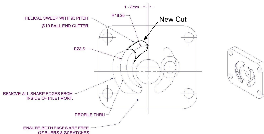
Figure 80 – Modified Port Details
