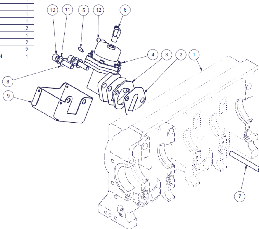
FUEL PUMP ASSY & MOUNTING
