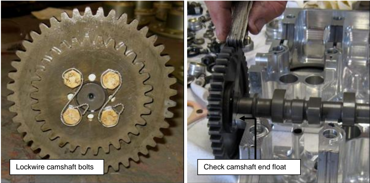
Figure 133 – Assembling Cam & Fitting to Crankcase
