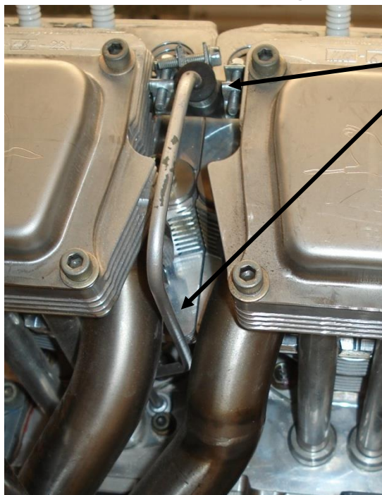
Figure 196 – Rocker Lube (Left) &amp; Crankcase Oil Port Blanking Plug
