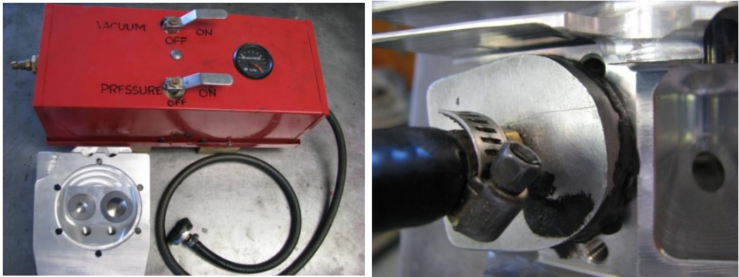
Figure 12 – Valve Leakage Vacuum Tester
