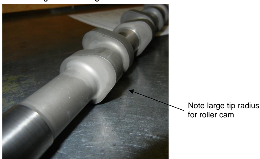
Figure 78 – Roller Cam Lobe
