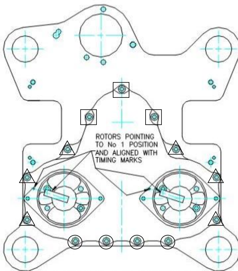
Figure 181 – Gearbox Installation
