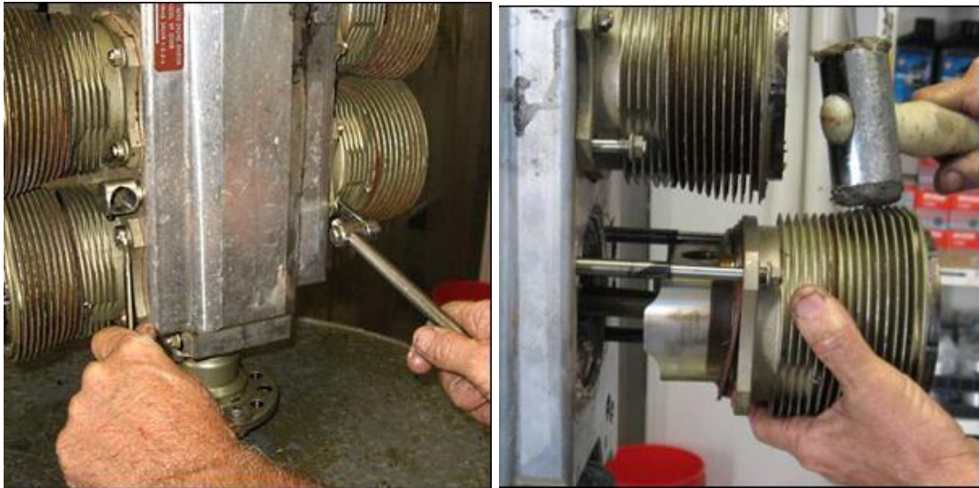
Figure 54 – Remove Cylinders
