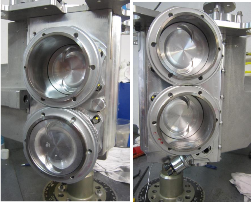
Figure 165 – Piston Orientation
