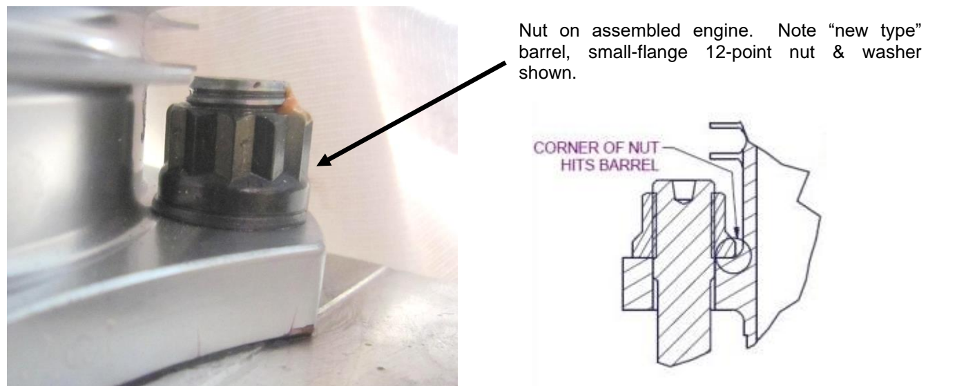
Figure 145 – Through Bolt Nut Installation Detail
