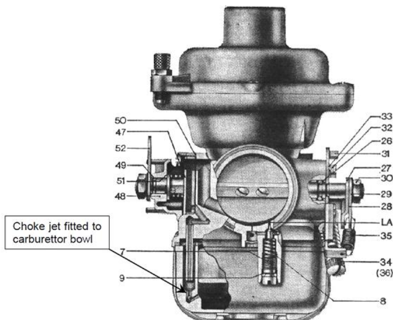
Figure 15 – Choke Schematic
