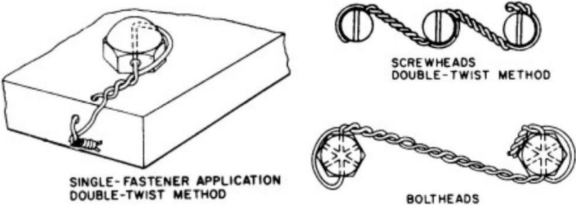
Figure 13 – Safety Wire Details
