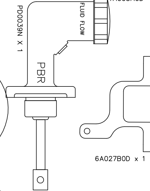
Brake Lever Stop cover x 1 1A003A0D
